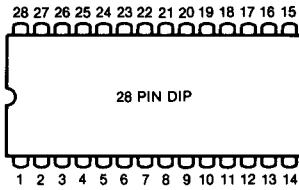
Fig. D-7. 28-pin dual in-line package.
